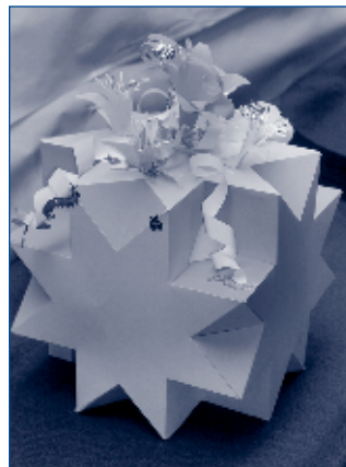
Polyhedral models built by students in Ginny Bohme's Geometry classes at Tucson High School
